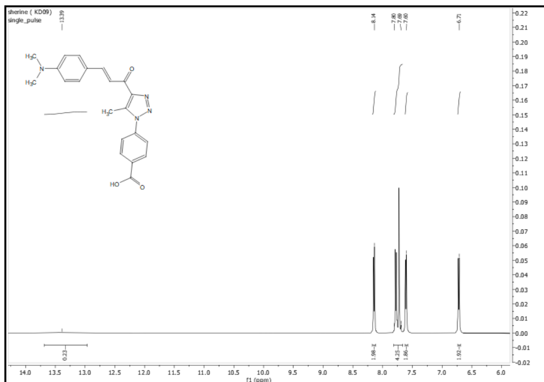
Figure S3: 1 H-NMR (500 MHz, DMSO- d 6 ) spectrum of ( E )-4-(4-(3-(4-(dimethylamino)phenyl)acryloyl)-5-methyl-1 H -1,2,3-triazol-1-yl)benzoic acid 3
