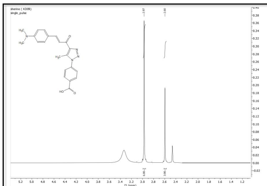
Figure S4: 1 H-NMR (500 MHz, DMSO- d 6 ) spectrum of ( E )-4-(4-(3-(4-(dimethylamino)phenyl)acryloyl)-5-methyl-1 H -1,2,3-triazol-1-yl)benzoic acid 3
