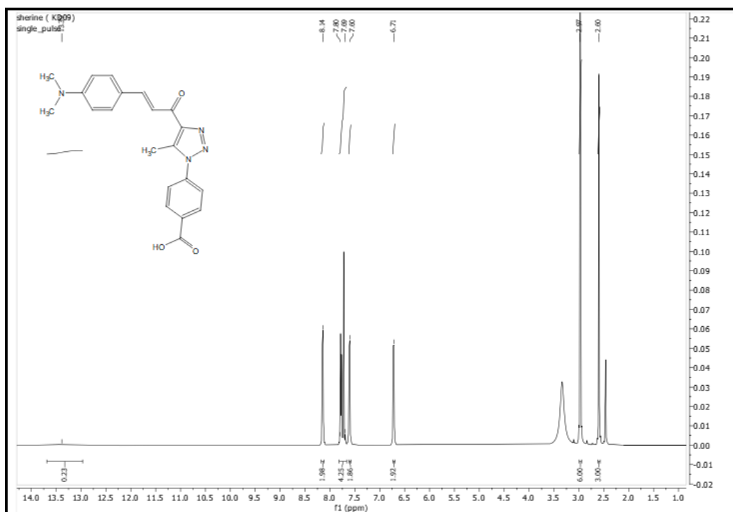
Figure S2: 1 H-NMR (500 MHz, DMSO- d 6 ) spectrum of ( E )-4-(4-(3-(4-(dimethylamino)phenyl)acryloyl)-5-methyl-1 H -1,2,3-triazol-1-yl)benzoic acid 3
