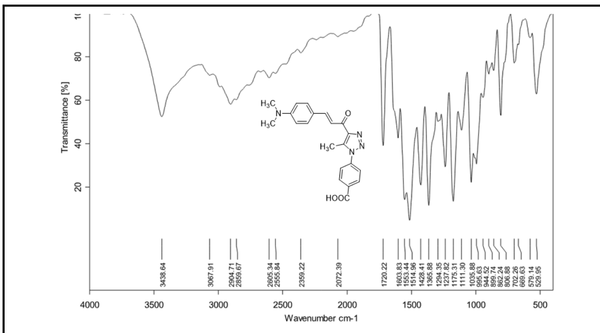
Figure S1: IR (KBr) spectrum of ( E )-4-(4-(3-(4-(dimethylamino)phenyl)acryloyl)-5-methyl-1 H -1,2,3-triazol-1-yl)benzoic acid 3
