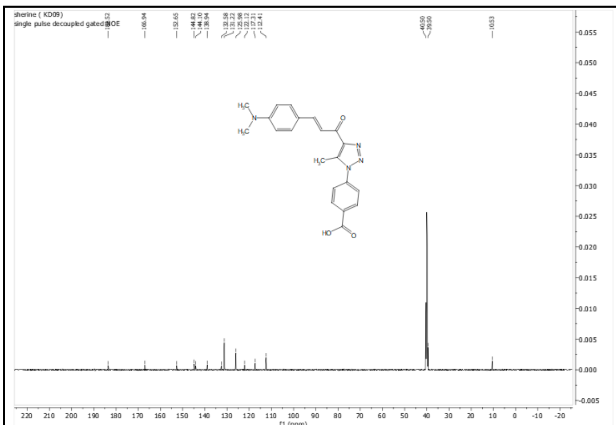
Figure S5: 13 C-NMR (125 MHz, DMSO- d 6 ) spectrum of ( E )-4-(4-(3-(4-(dimethylamino)phenyl)acryloyl)-5-methyl-1 H -1,2,3-triazol-1-yl)benzoic acid 3
